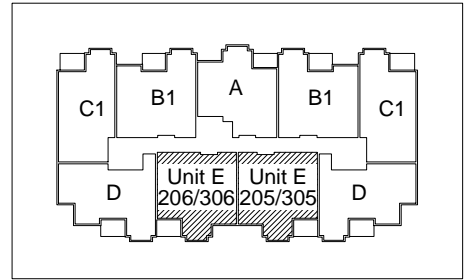
SECOND & THIRD FLOOR
